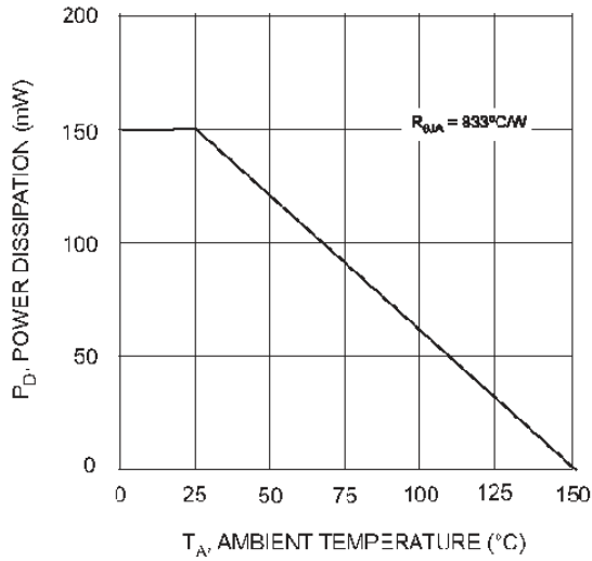
Fig. 1 Derating Curve
