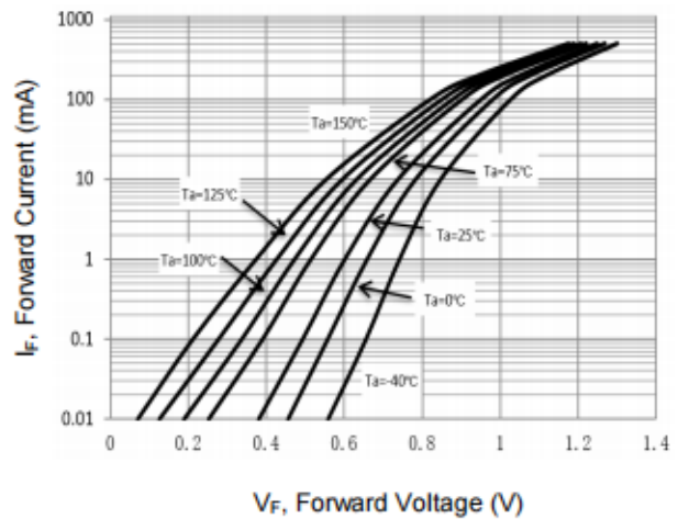
Fig 4. Forward Characteristics
