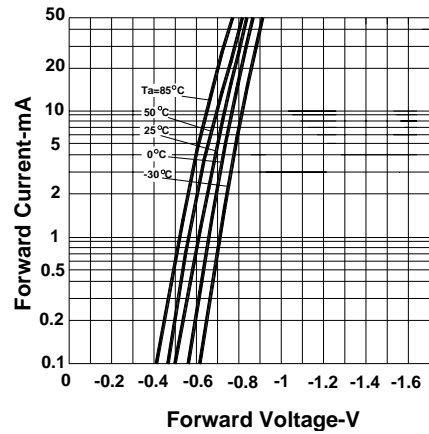
Forward Characteristics
