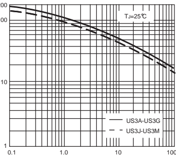
FIG. 5-TYPICAL JUNCTION CAPACITANCE
